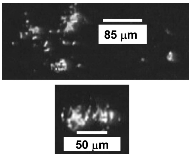
FIGURE 4 Optical polarizing microscope images of planar-aligned liquid crystal cells after laser irradiation, showing one/two/three spots of destroyed planar alignment.
