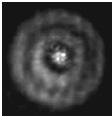
FIGURE 3 Far-field pattern of two polarization components with four-leaf-clover pattern of the “perpendicular” polarization component overlapped with the fringes of the “parallel” polarization component.
